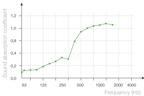
Sound absorption characteristics for 28 mm panel
